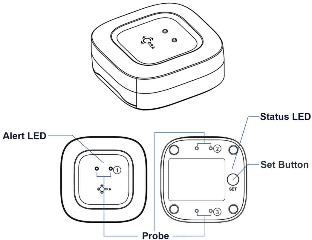
Figure 1 – CS1010 Leak Sensor
